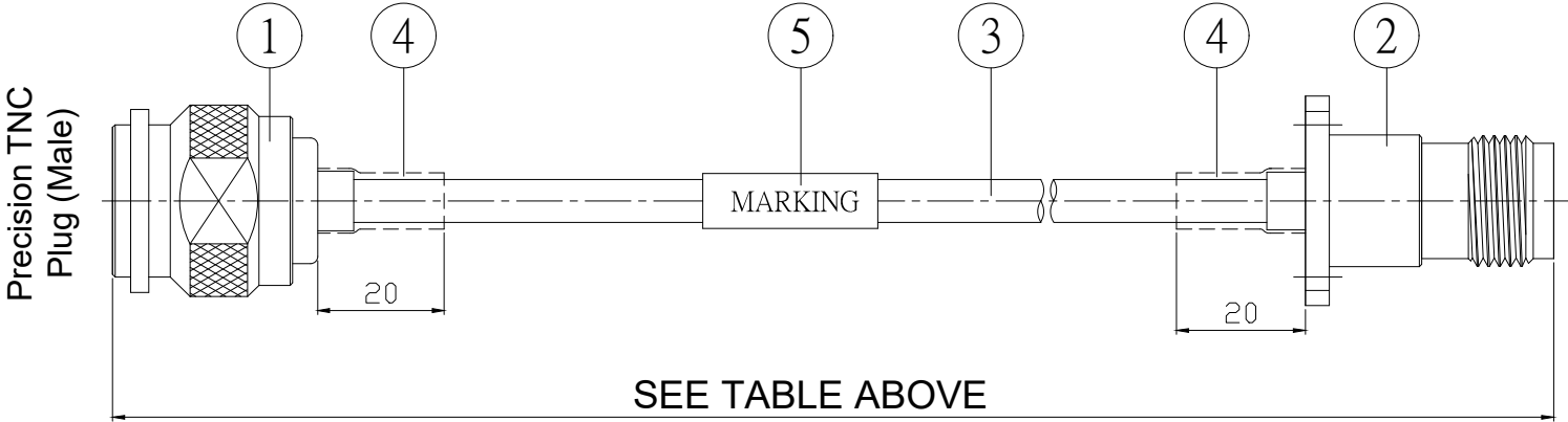
Precision TNC Panel Jack (Female)
