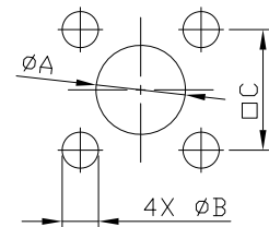
Mounting Dimensions
