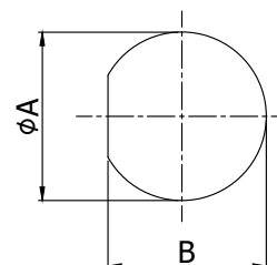
Mounting Dimensions
