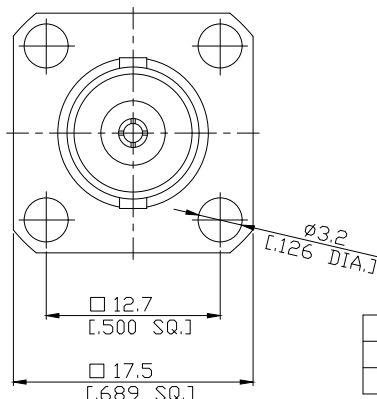
Mounting Dimensions
