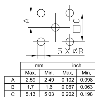
Mounting Dimension
