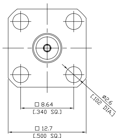
Mounting Dimensions
