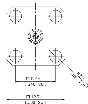
Mounting Dimensions
